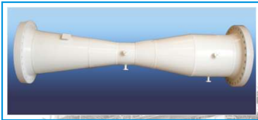
Size : 42 inch dia; 7.4 meter long fabricated Venturi Meter
